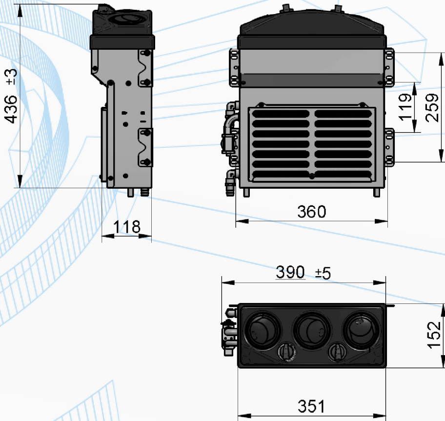
HVAC Unit
