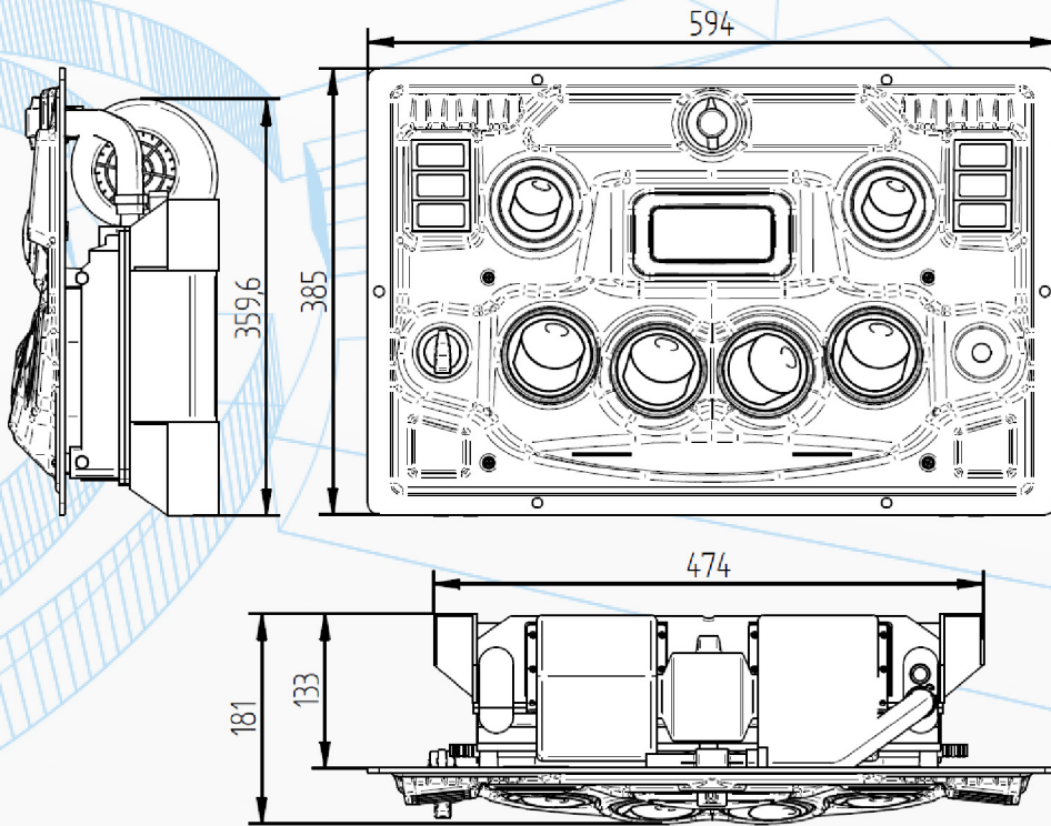
HVAC Unit
